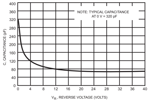
FIG.6- TYPICAL CAPACITANCE
